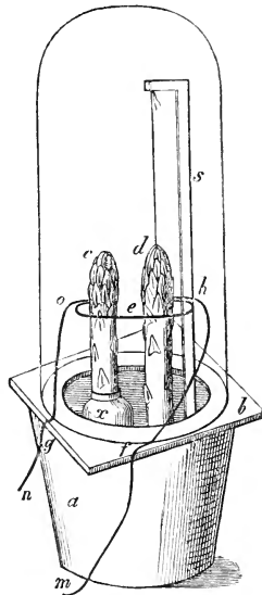
FIG. 66. Apparatus for thermo-electric measurement of temperature: ( c ) living, ( d ) dead shoot; ( e ) German-silver wire; ( m and n ) iron wire; at o and e the thermo-electric junctions are inserted in the shoots.
